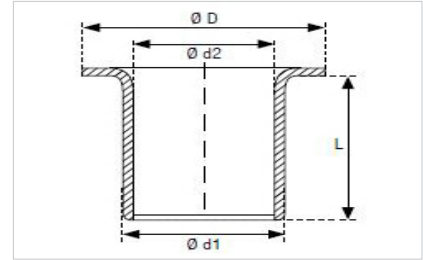
Standard Eyelet Dimensions
